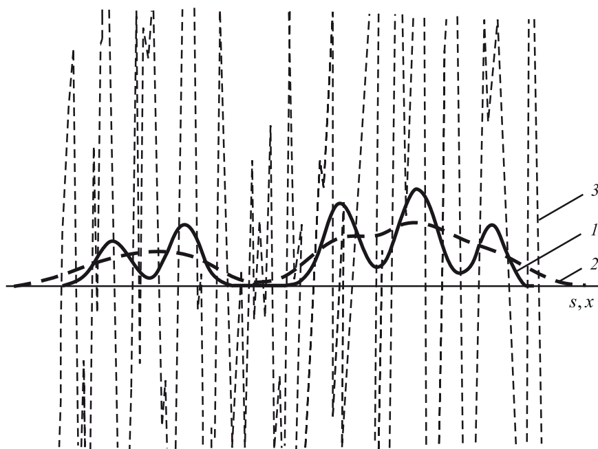
Figure 4.2. Instable solution of the Fredholm integral equation of the first kind obtained by the quadrature method:
